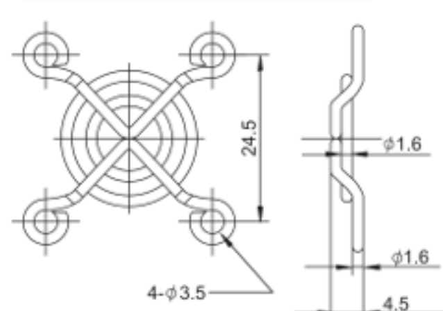
FG-03 For 30mm Fan
