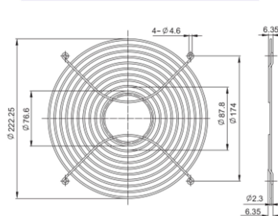
FG-25 For 254mm Fan
