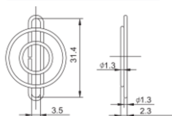
FG-02 For 25mm Fan
