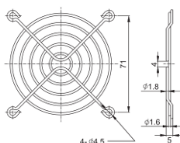
FG-08 For 80mm Fan
